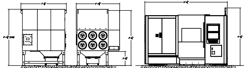
Dust Collector
