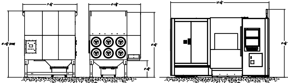
Dust Collector
